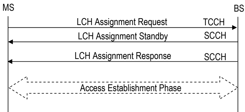
Figure 8.16 Link Channel Assignment Standby Sequence
