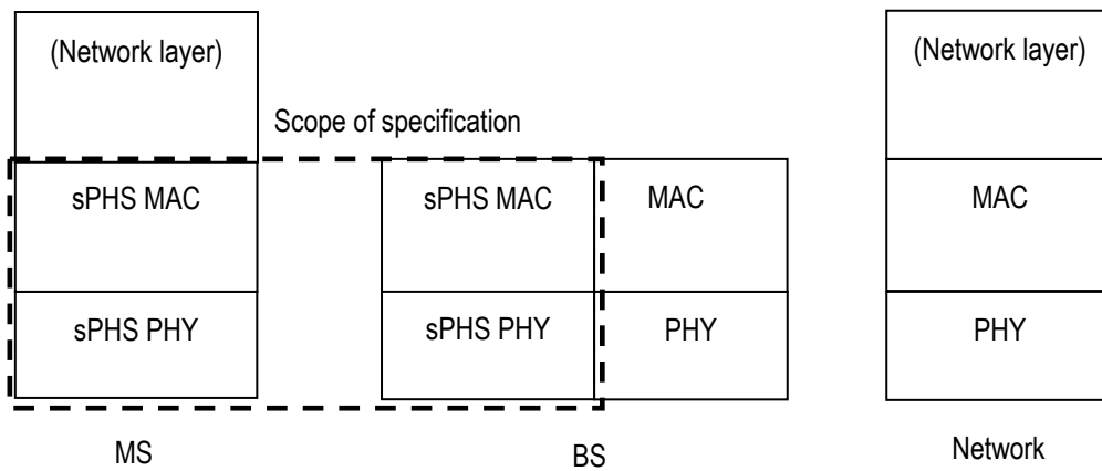
Figure 2.14 Protocol Stack for sPHS
