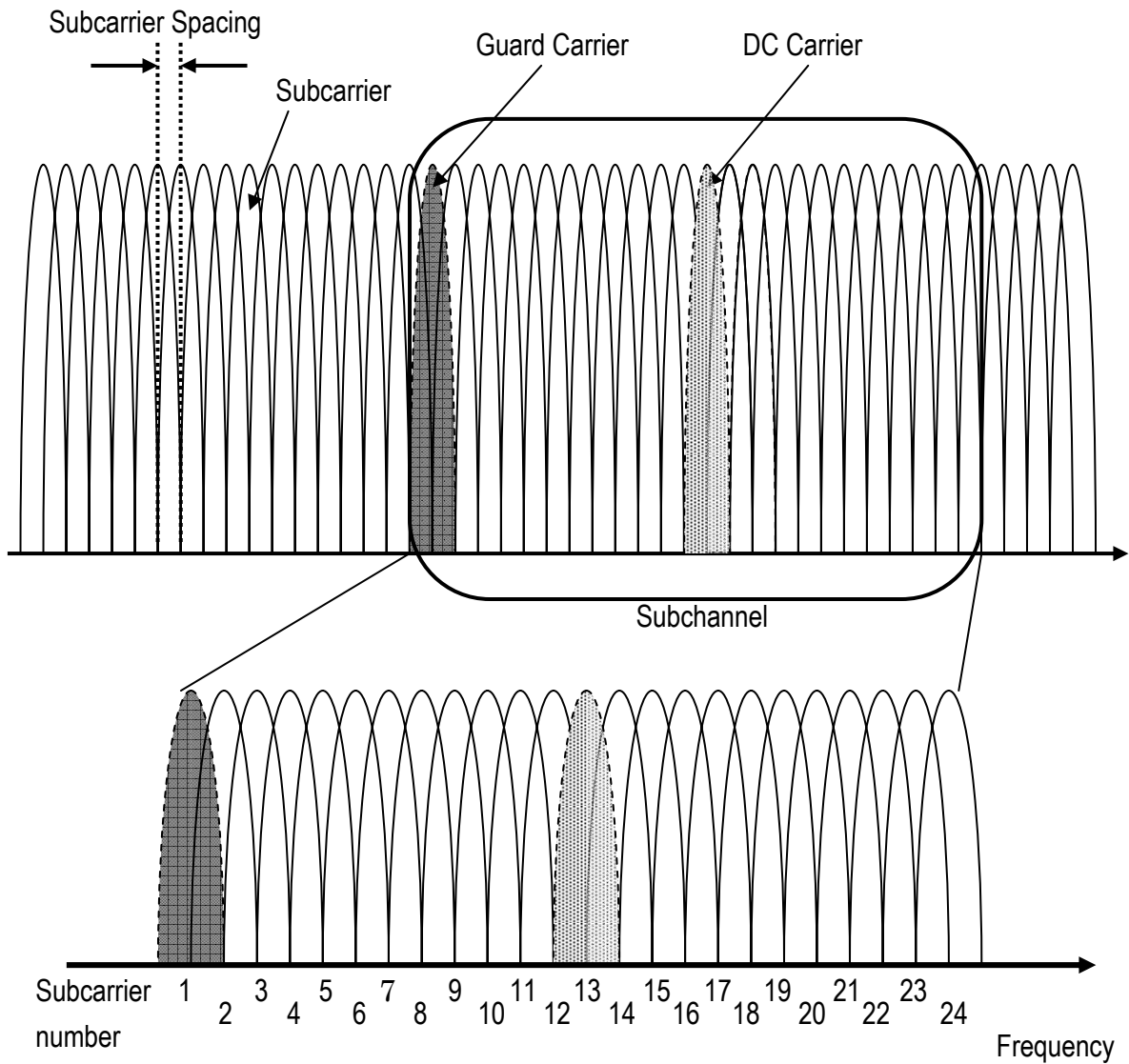
Figure 2.5 OFDMA Structure
