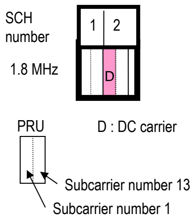
Figure A.1 Full Subcarrier Mode
