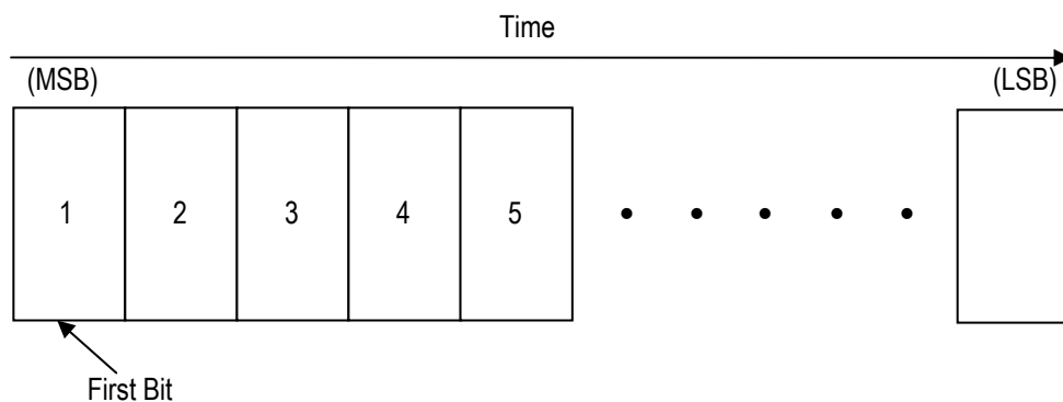
Figure 4.33 Correspondence between Logical PRU Number and Bit Position in the MAP Field
