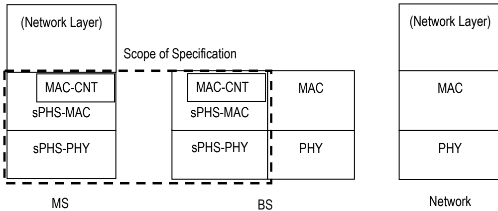
Figure 4.6 Protocol Stack for sPHS (MAC Control)
