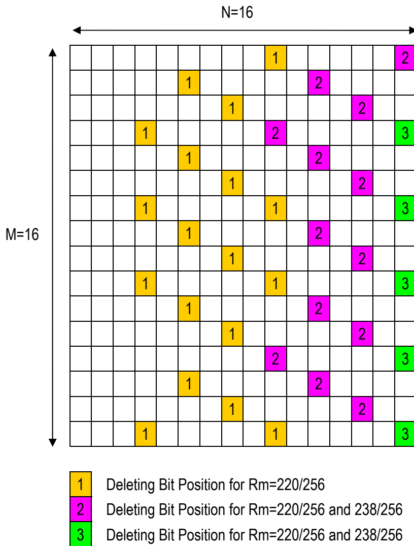
Figure 3.63 Deleting Bit Position of ICH: Pattern B2
