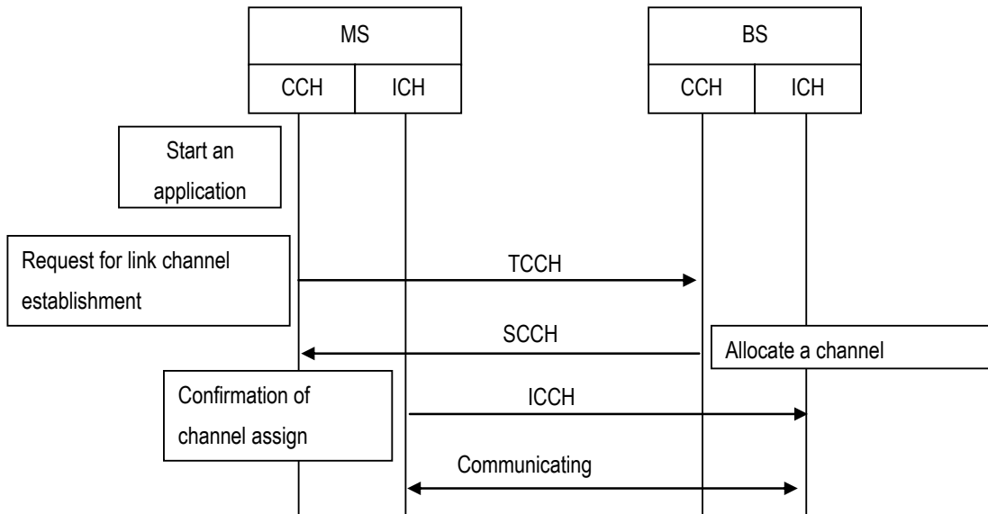
Figure 6.2 Outgoing Call Sequence
