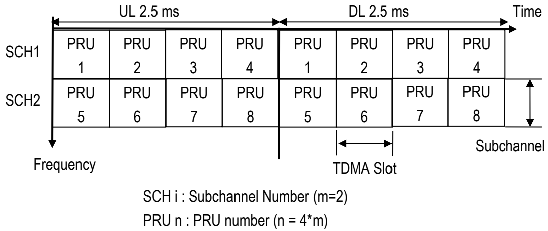
Figure 2.10 Correspondence between Subchannel Number and PRU Number
