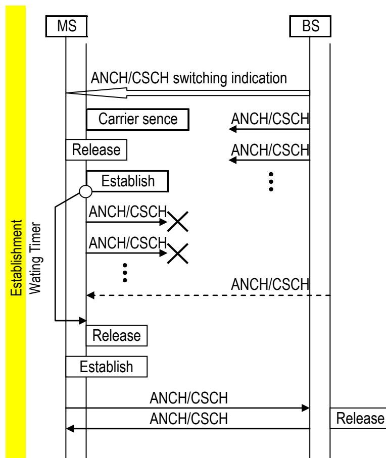
Figure 9.33 ANCH/CSCH Switchback
