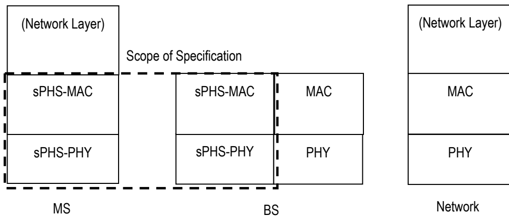
Figure 4.5 Protocol Stack for sPHS
