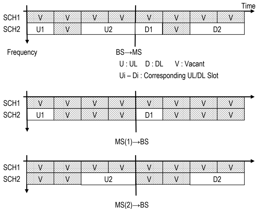
Figure 2.8 OFDMA/TDMA Slot Arrangement
