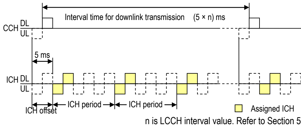
Figure 5.5 Intermittent Transmission Timing for ICH
