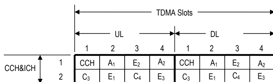
Figure 4.2 Example of ICH Usage
