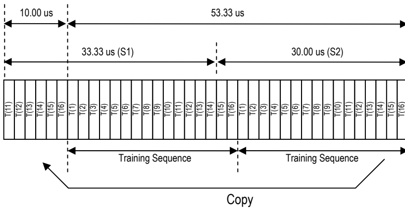
Figure 3.70 Training format for CCH
