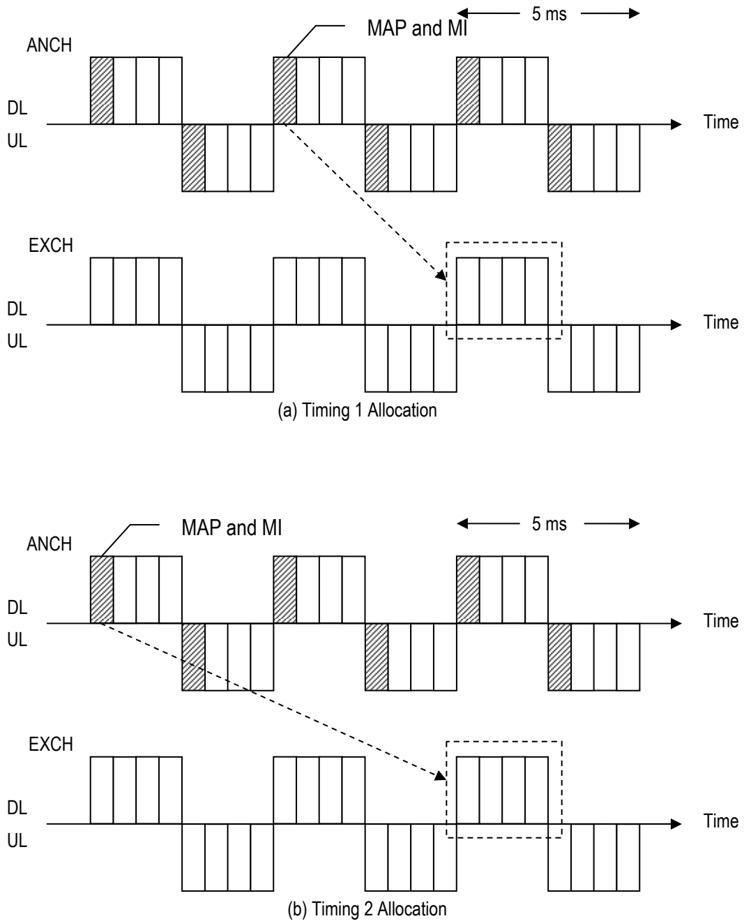
Figure 4.23 Example of DL MI Indication Timing in ECCH
