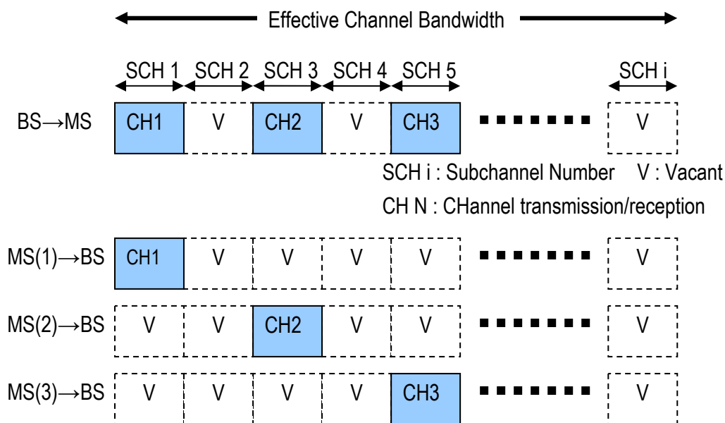
Figure 2.6 OFDMA Frequency Arrangement
