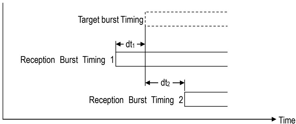
Figure 9.22 Time Difference Between Target Timing and Reception Timing
