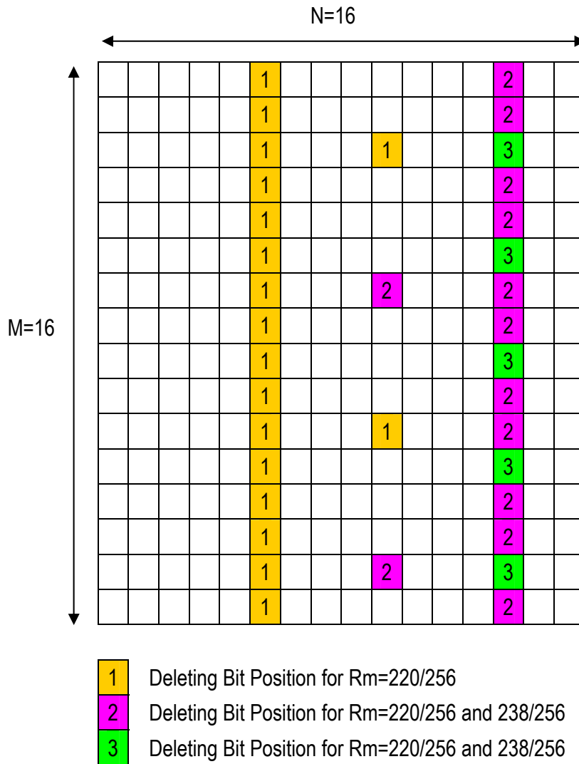
Figure 3.61 Deleting Bit Position for ICH: Pattern A
