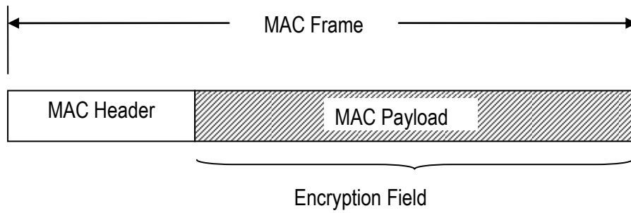
Figure 9.41 Encryption Field
