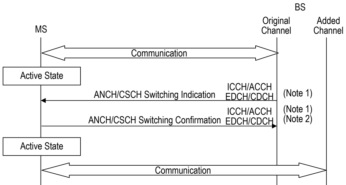
Figure 8.9 ANCH/CSCH Switching Triggered by BS Sequence
