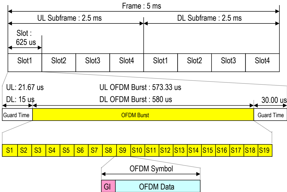
Figure 3.1 OFDM Symbols
