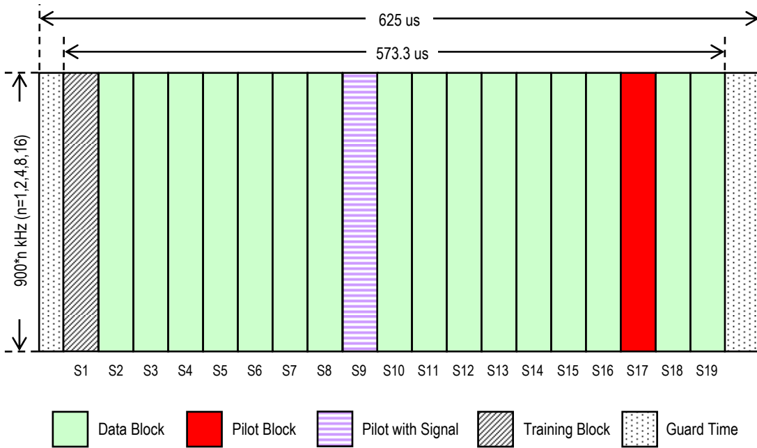
Figure 3.80 SC Burst Structure for CSCH
