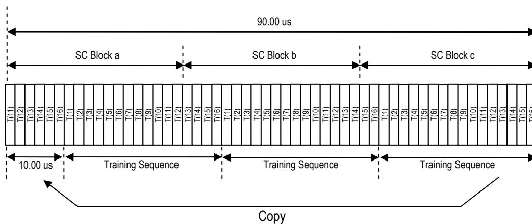
Figure 3.75 TCCH Block Structure
