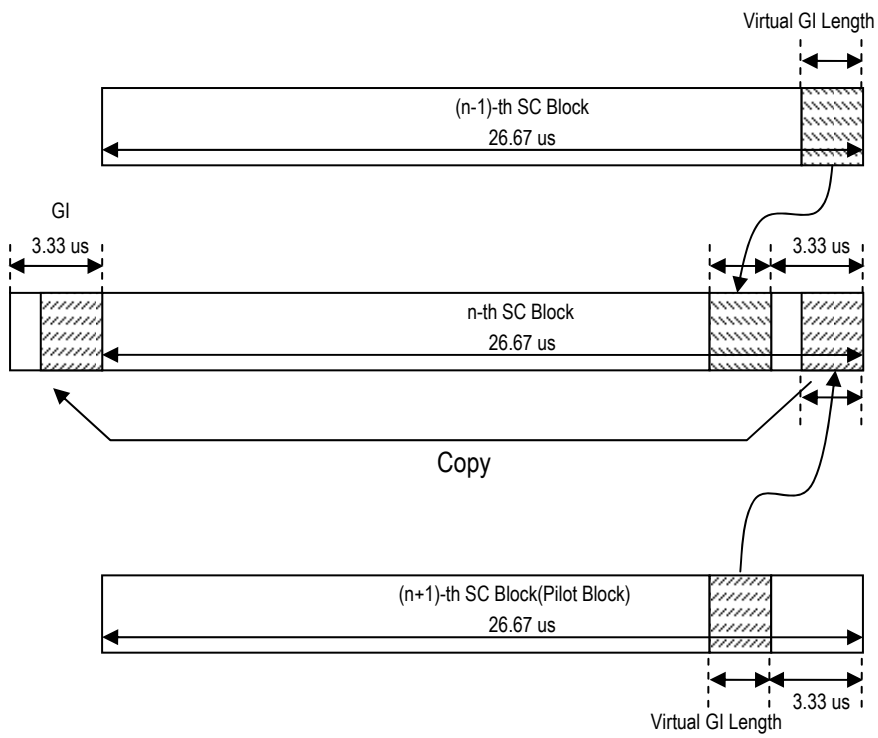
Figure 3.68 Symbol Mapping of SC Block with Virtual GI Extension (S8 and S16)
