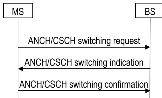
Figure 9.28 MS Origin ANCH/CSCH Scheduling Change
