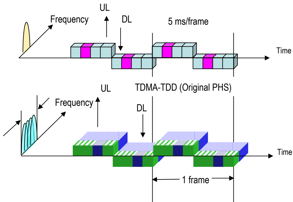
Figure 2.3 OFDMA/SC-FDMA/TDMA-TDD (sPHS)
