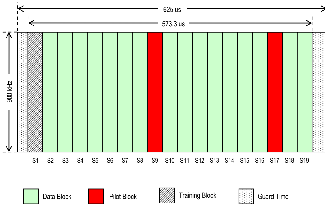
Figure 3.78 SC Burst Structure for ANCH
