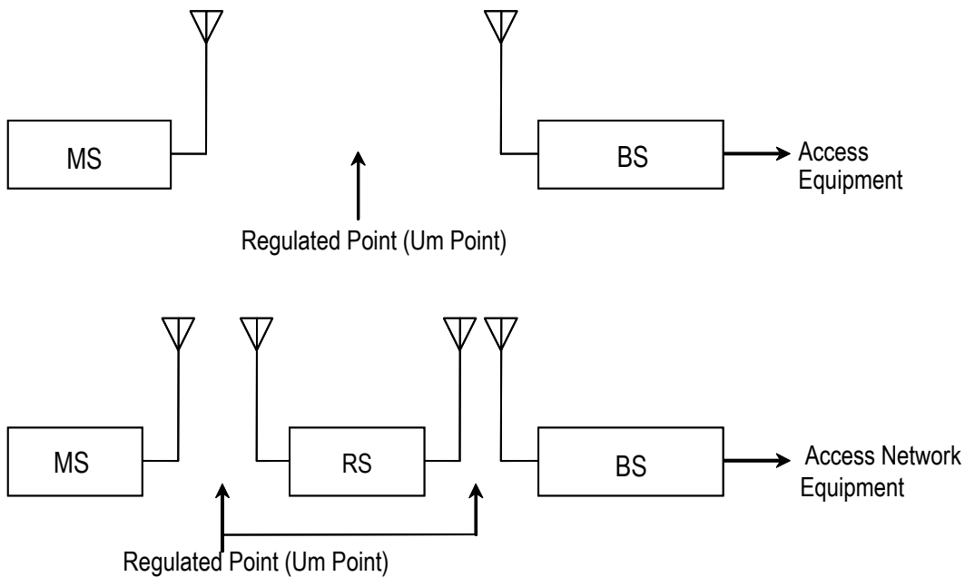
Figure 1.1 Structure of sPHS
