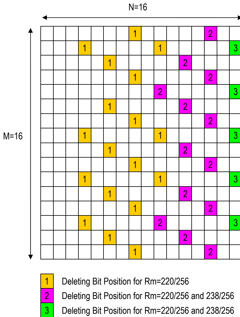
Figure 3.62 Deleting Bit Position for ICH: Pattern B1
