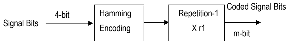
Figure 3.73 Signal Encoding for SC
