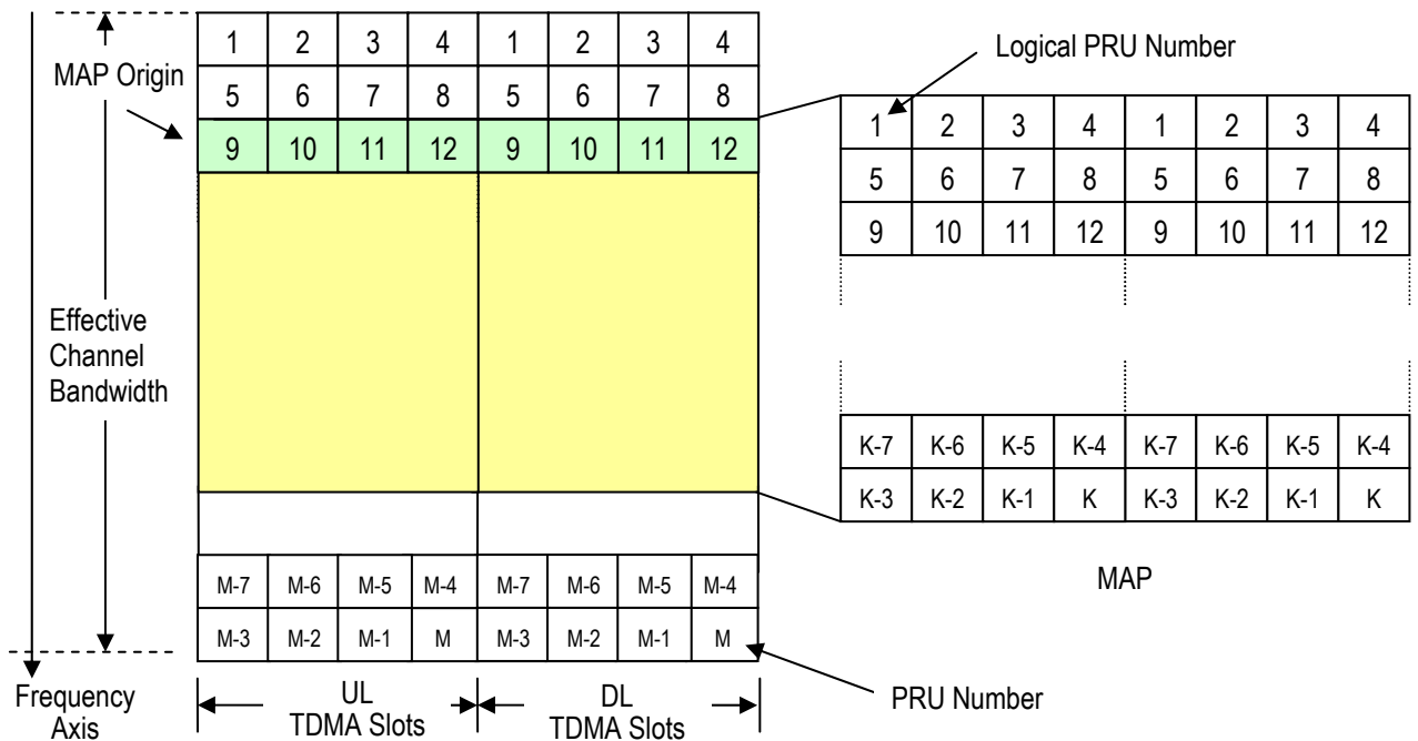
Figure 4.32 Logical PRU Numbering
