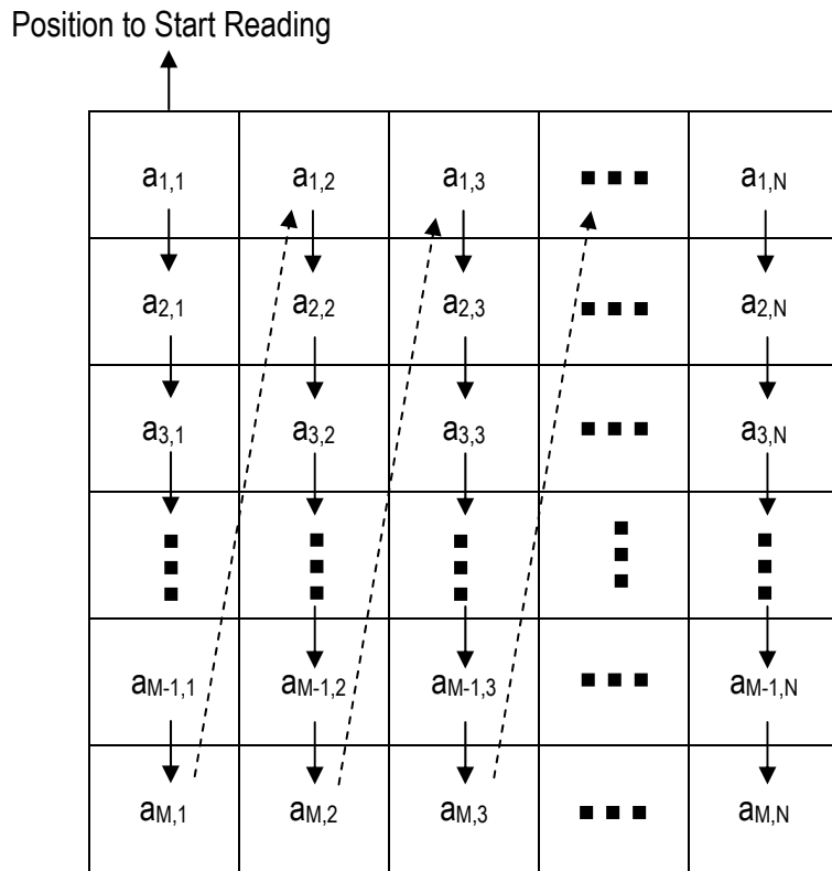
Figure 3.28 Interleaver Matrix (Read-out) in case of n being 1
