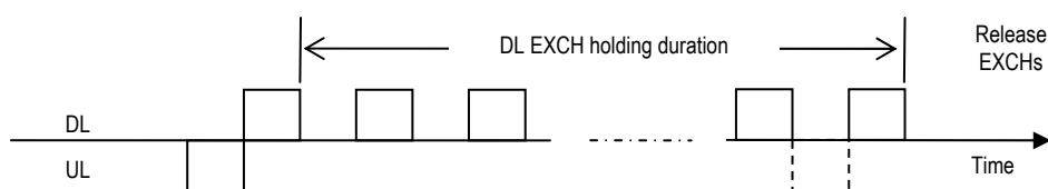
Figure 6.11 EXCH Release Timing
