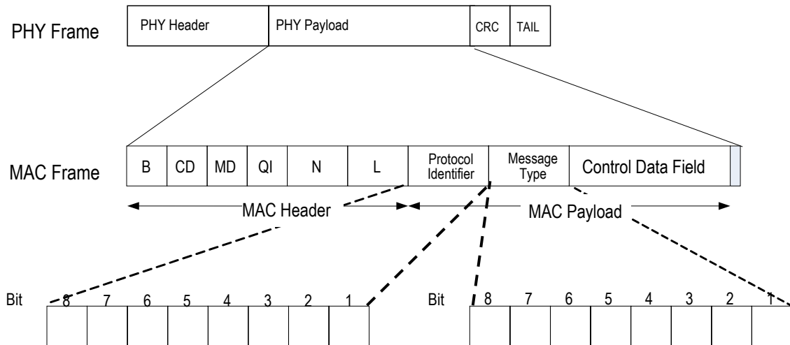
Figure 4.69 Relation among MAC Control Information, MAC Frame and PHY Frame
