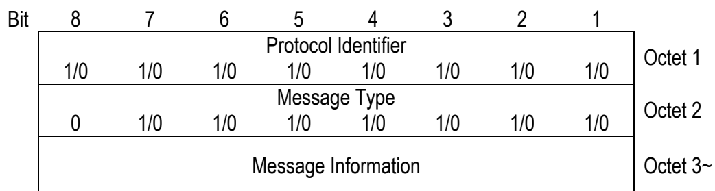
Figure 7.1 Message Format
