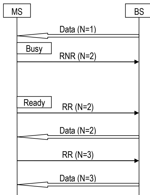
Figure 9.36 RNR Used in Flow Control
