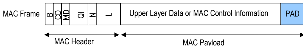
Figure 4.51 A General MAC Frame Structure (Included MAC Header)
